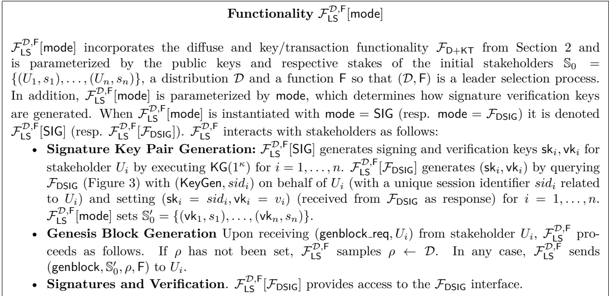
Figure 1: Functionality \mathcal{F}_{\text{LS}}^{\mathcal{D}, F}[\text{mode}] .
