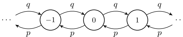
Figure 6: The simple biased walk where p = (1 + \epsilon)/2 and q = 1 - p .
